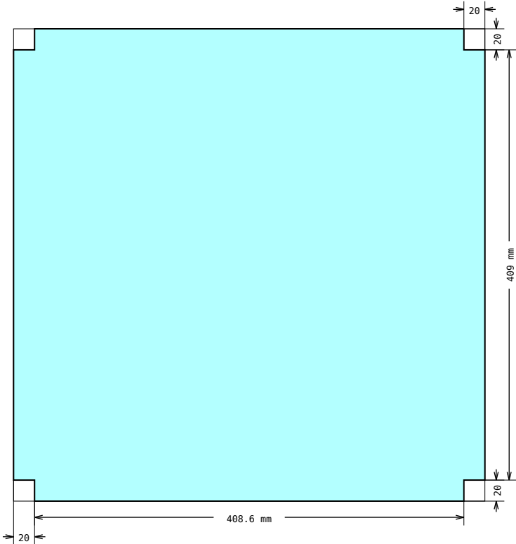
DRAWING 1, Pos 5 Shape measurements
